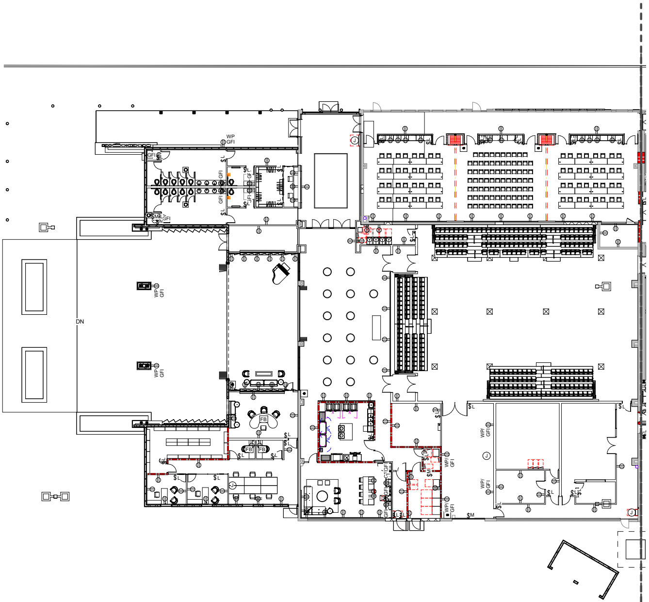
FIRST FLOOR FURNITURE PLAN COMPOSITE 1/16" = 1'-0"
